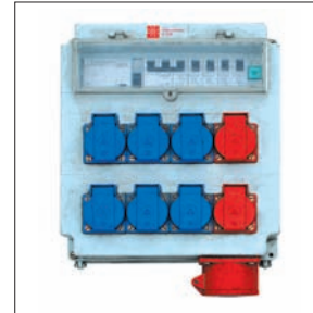
Electrical panel OCTANORM Code 019.010.275.000 EUR 120.00
